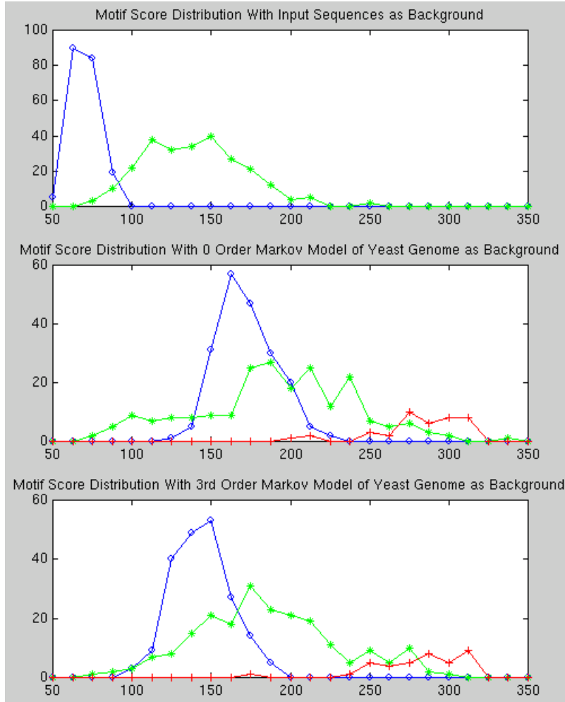
Figure 2. Motif scores of the RAP1-binding data. The top, middle and bottom plots show the motif score distribution using input sequence F_m , a zero-order, and a third-order Markov model estimated from yeast intergenic region as the background, respectively. The three curves with 'o' data points represent the motif score distribution of the 200 generated sequence sets and all 3 curves approximate a normal distribution. The score distribution of the 250 motifs found from original input sequences are shown in '*' and '+'. The curve with '*' data points represents the false positive motif scores and the curve with '+' data points represents the true positive motif scores. With a third-order Markov background model estimated from yeast intergenic region, all the motifs with a score above 305 are correct.
